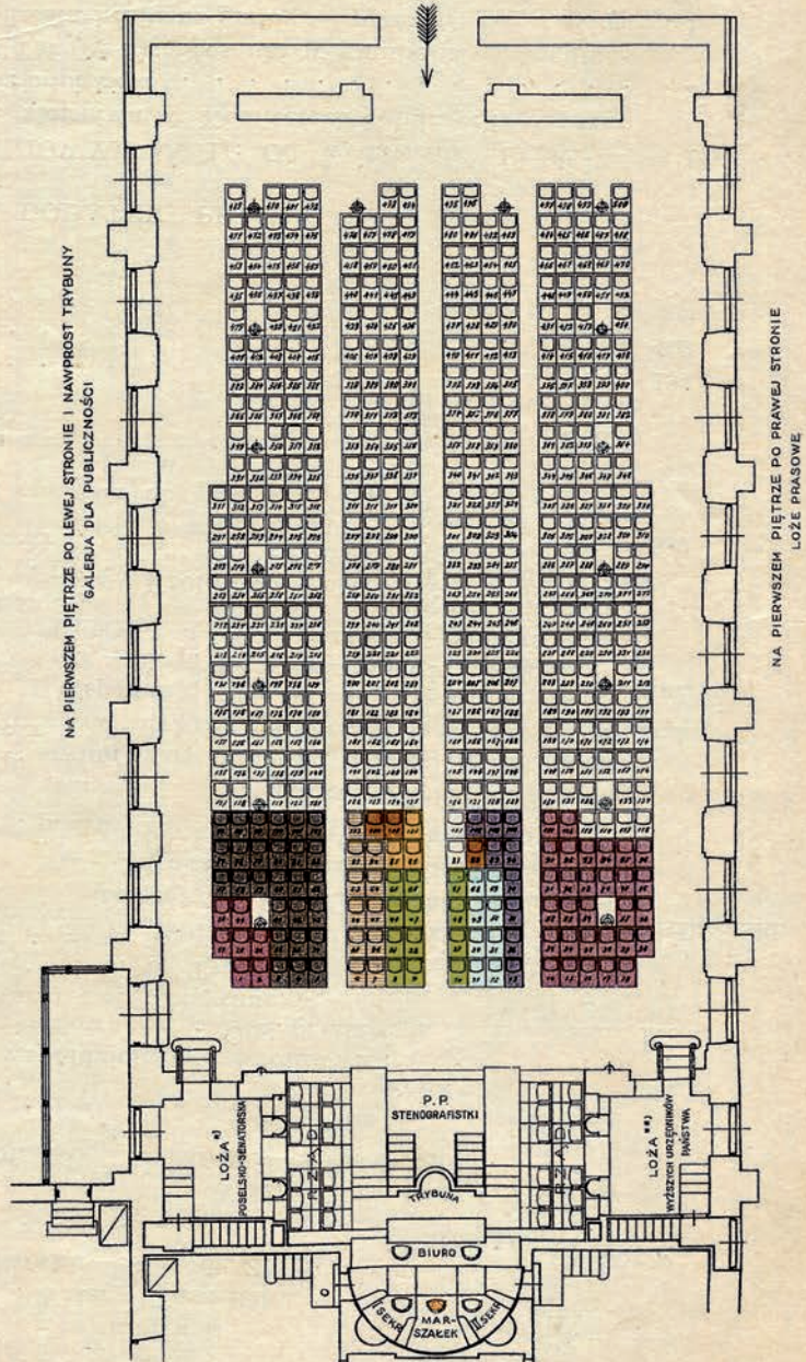
PLAN PARTERU
