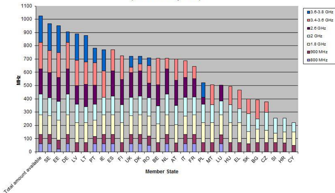
Assigned spectrum in EU harmonised bands (status: 25 July 2013)
